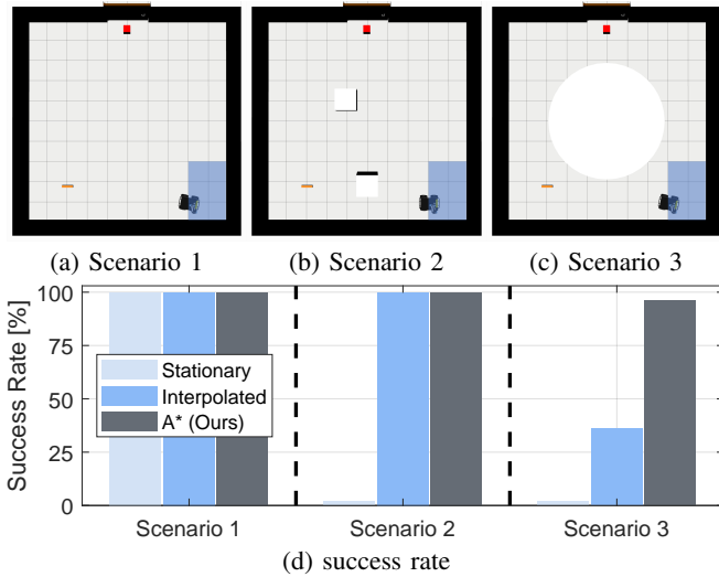
Fig. 3: Comparisons of motion planning on VKCs by different trajectory initialization methods. (a)-(c) The experimental scenarios in increasing complexity. The robot’s initial pose is uniformly sampled within the blue region; it is tasked to pick up the stick and use it to reach the red cube. (d) The proposed A*-based trajectory initialization has the highest success rates (almost always) in generating a feasible plan. In comparison, the Stationary method fails to generate feasible plans in scenario 2 and 3. Similarly, the Interpolated method struggles in scenarios 3 (30% success rate).
