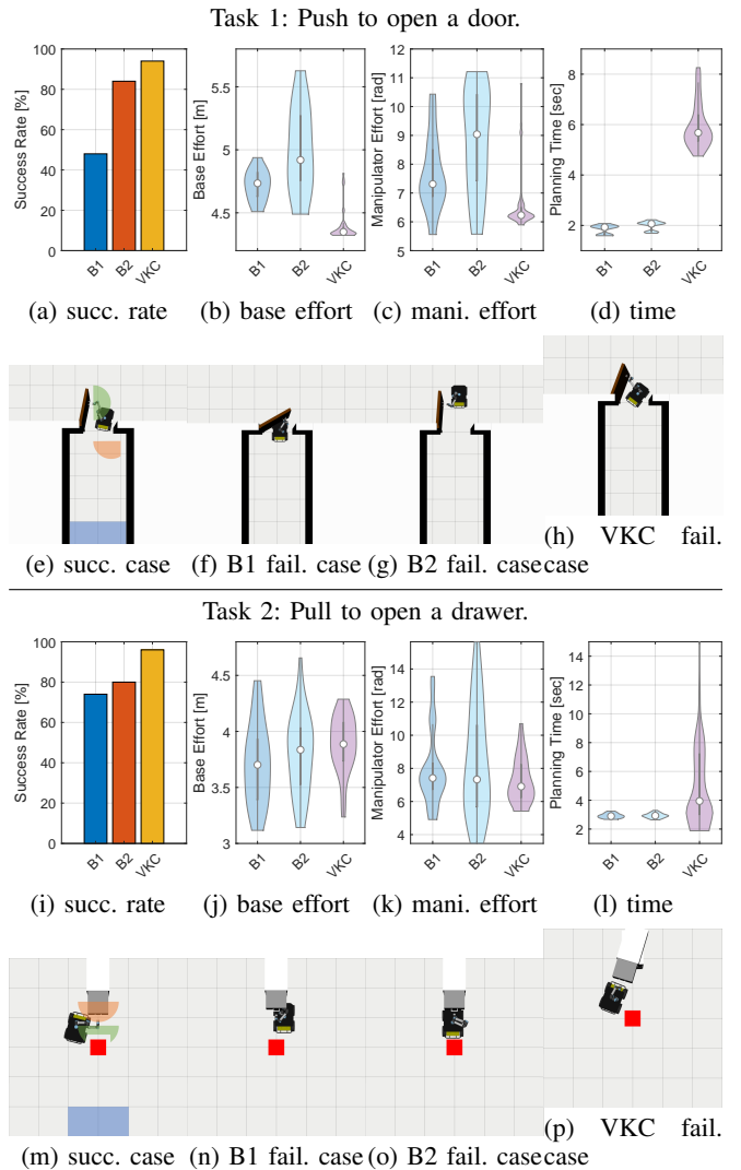
Fig. 4: Quantitative comparisons between the VKC-based approach and two baselines on two mobile manipulation tasks: push to open a door, and pull to open a drawer. Modeling a mobile manipulation using VKC leads to (a)(i) higher success rate and more effective trajectories in terms of smaller (b)(j) base and (c)(k) manipulator’s efforts, but requires (d)(l) longer planning time. Of note, baselines require additional definition of intermediate goals, which are often empirically found, (e)(m) shown in the green and pink shaded areas. (f)(n) Typical failure cases of two tasks in B1 are due to collision. Typical failure cases of two tasks in B2 or (h)(p) VKC-based approach are due to constraint violations.
