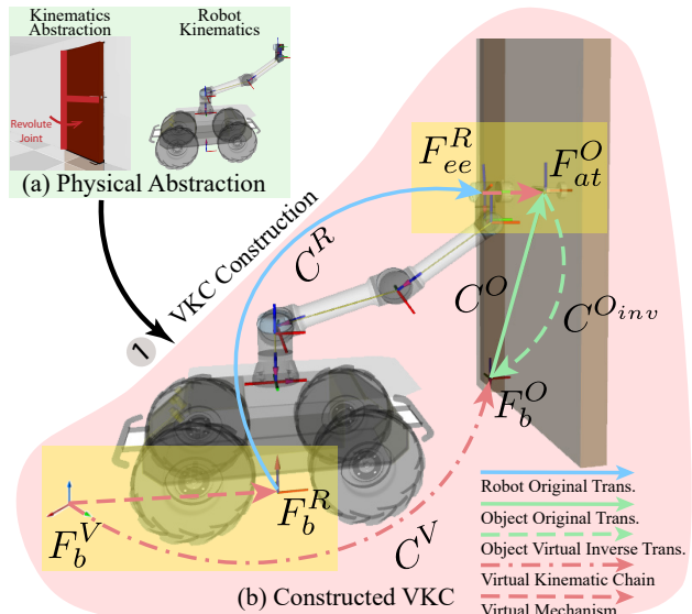
Fig. 2: Overview of the mobile manipulation planning schematics using the proposed VKC-based approach. (a) After abstracting out the underlying kinematics of the manipulated object and the mobile manipulator, (b) a VKC is constructed. The yellow boxes denote where the virtual connections are established: (i) One between \mathcal{F}_b^V and \mathcal{F}_b^R , the virtual base frame in the world coordinate and the robot’s actual base frame, to reflect the navigational information, and (ii) another between \mathcal{F}_{ee}^R and \mathcal{F}_{at}^O , the robot’s end-effector frame and the attachable frame of the object, to transfer effects of the manipulator to the manipulated object.
