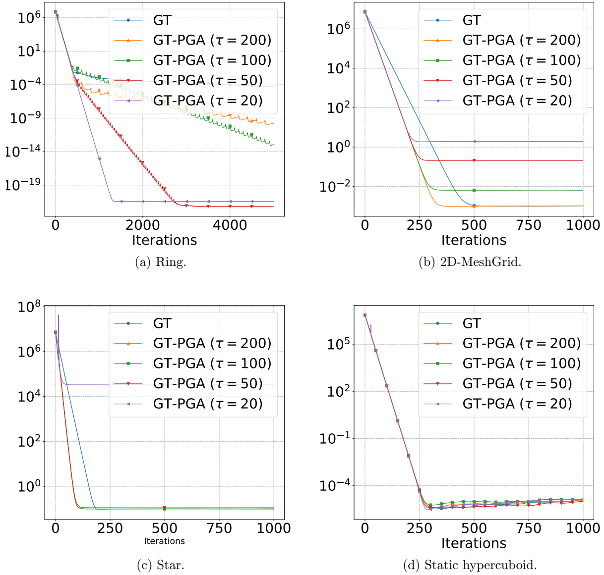
Figure 1: Performance of GT-PGA for solving (13) with various topologies. The plots report \|\nabla \bar{f}(\bar{\mathbf{x}}^{(k)})\|^2 + \|\nabla f(\bar{\mathbf{x}}^{(k)})\|^2 , and use the ring, 2D-MeshGrid, the star graph, and the static hypercuboid, respectively. Different curves on each figure use different PGA period, i.e. , \tau = 20, 50, 100, 200 , and \infty (equivalent to vanilla GT).
